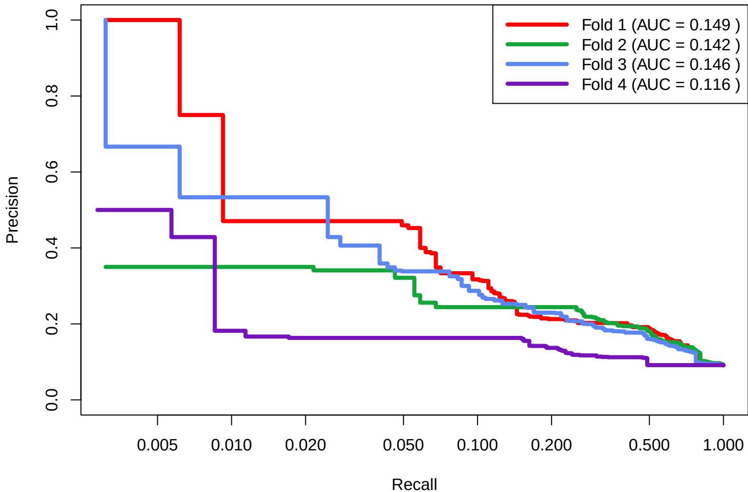
SPELL Original Datasets: 113x100x1 Validation
