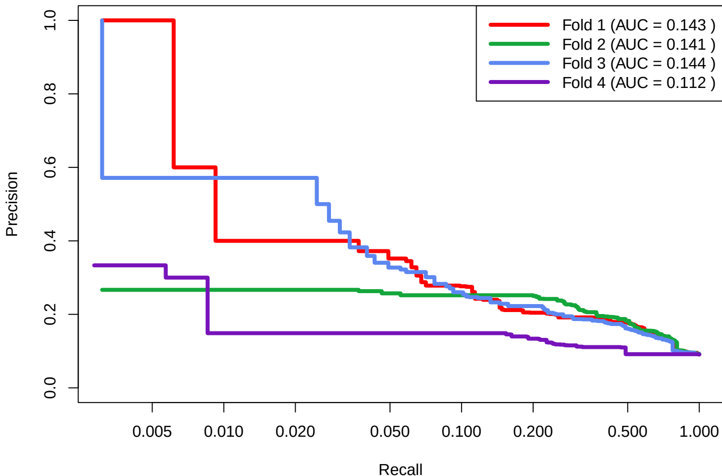
SPELL Original Datasets: 113x100x1 Training
