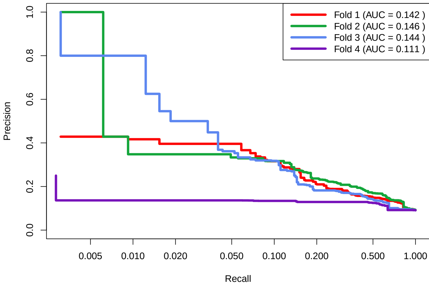
SPELL Original Datasets: 113x50x1 Training
